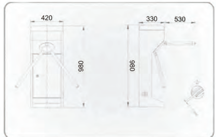
Vertical Type S-TVT
