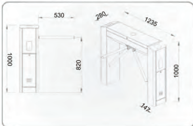
Bridge Type S-T200S
